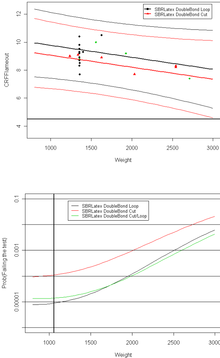
Figure 7-8: CRFFlamout vs Weight for SBRLatex and probability of failing the CRFFlamout test at 4.5kW
