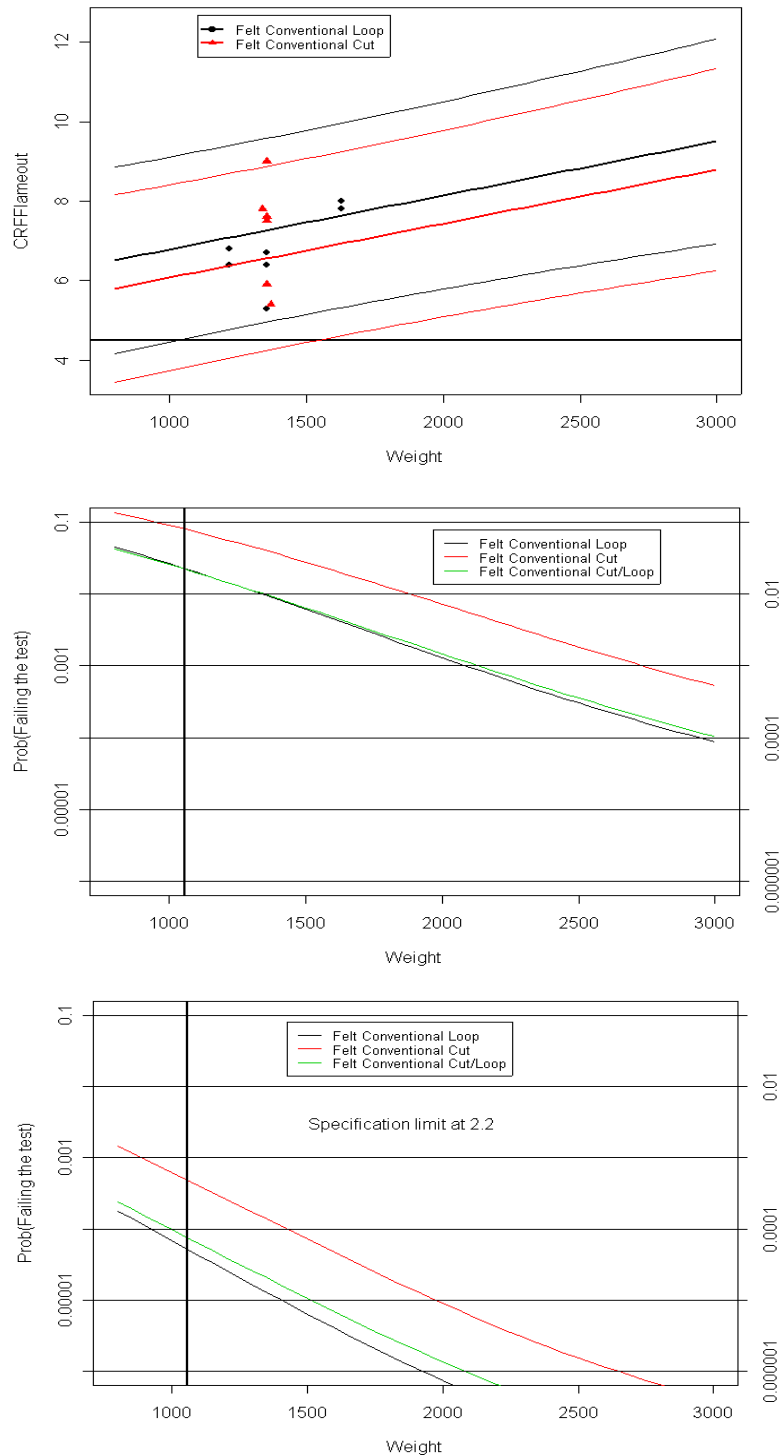
Figure 7-11: CRF vs Weight for Felt (top graph) and implied probability of failing the CRF test at 4.5 kW/m 2 (left graph) and 2.2 kW/m 2 (right graph).
