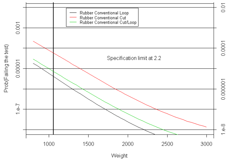
Figure 7-4: Implied probability of failing the CRF test at 2.2 kW/m 2 for Rubber
