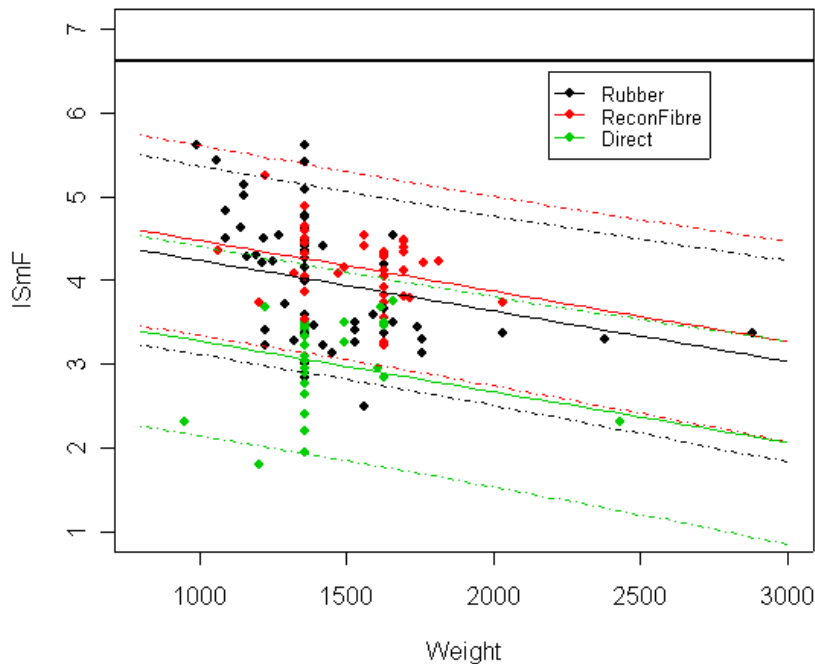
Figure 7-14: logSDR vs Weight, with fitted curves and 95% prediction intervals for first three classes.
