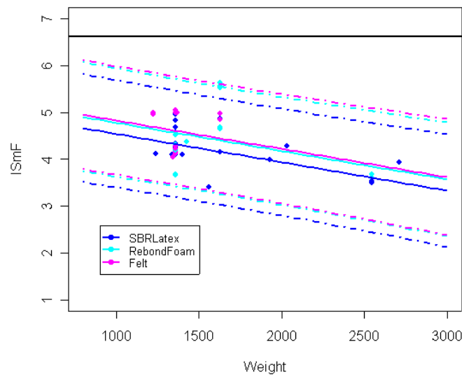
Figure 7-16: logSDR vs Weight, with fitted curves and 95% prediction intervals for another three classes.
