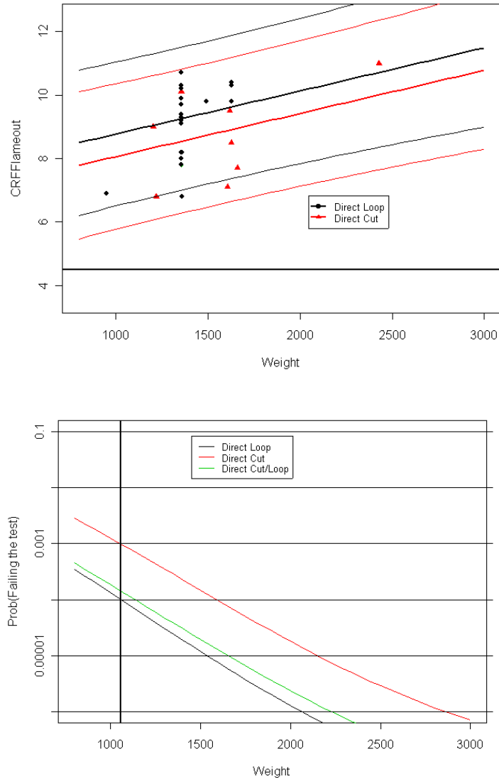
Figure 7-7: CRF vs Weight for Direct Stick and probability of failing the CRF test at 4.5 kW/m 2 .
