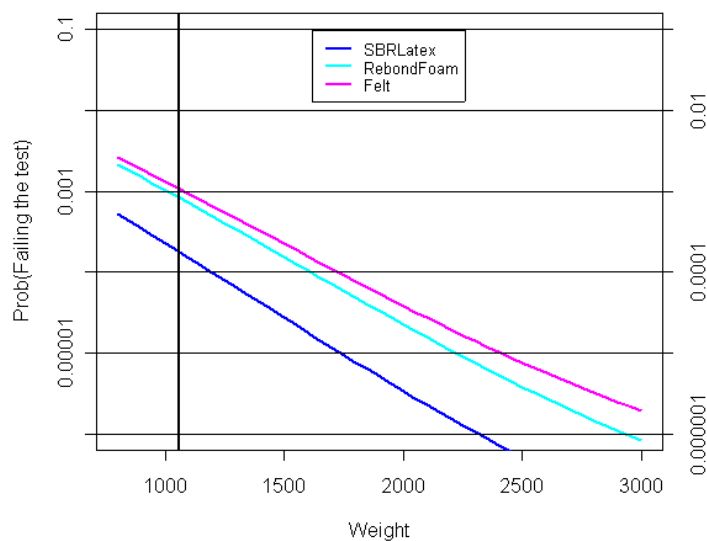
Figure 7-17: Probability of failing the SDR test, for the other three classes.
