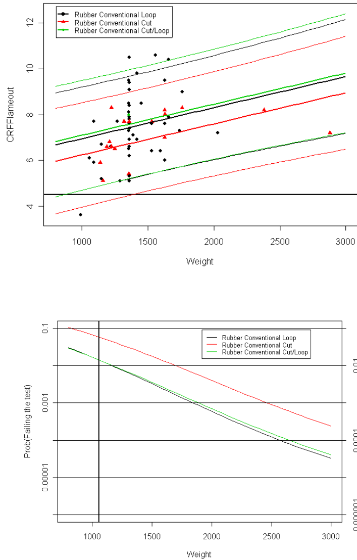
Figure 7-3: CRF vs Weight for Rubber with 95% prediction intervals; implied probability of failing the CRF test at 4.5 kW/m 2 .
