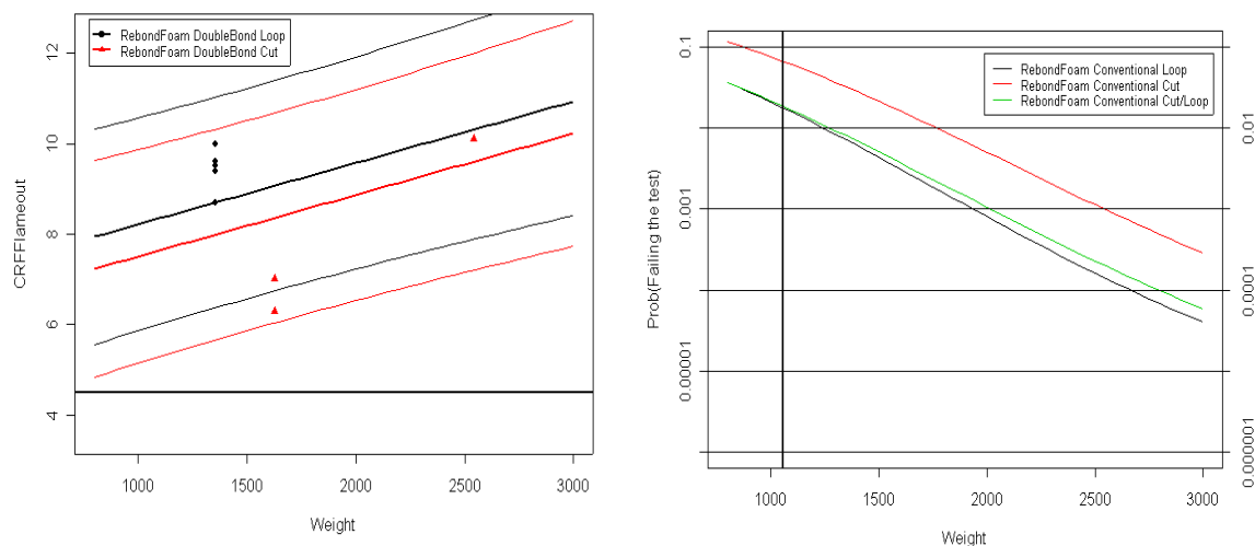
Figure 7-10: Implied probability of failing the CRF test at 2.2kW/m 2 for Rebond Foam, Conv and DoubleBond
