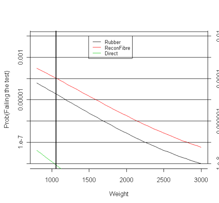
Figure 7-15: Probability of failing the SDR test, for first three classes.
