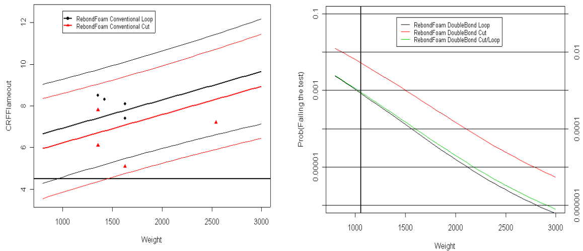
Figure 7-9: CRF vs Weight for Rebond foam and implied probability of failing the CRF test at 4.5 kW/m 2
