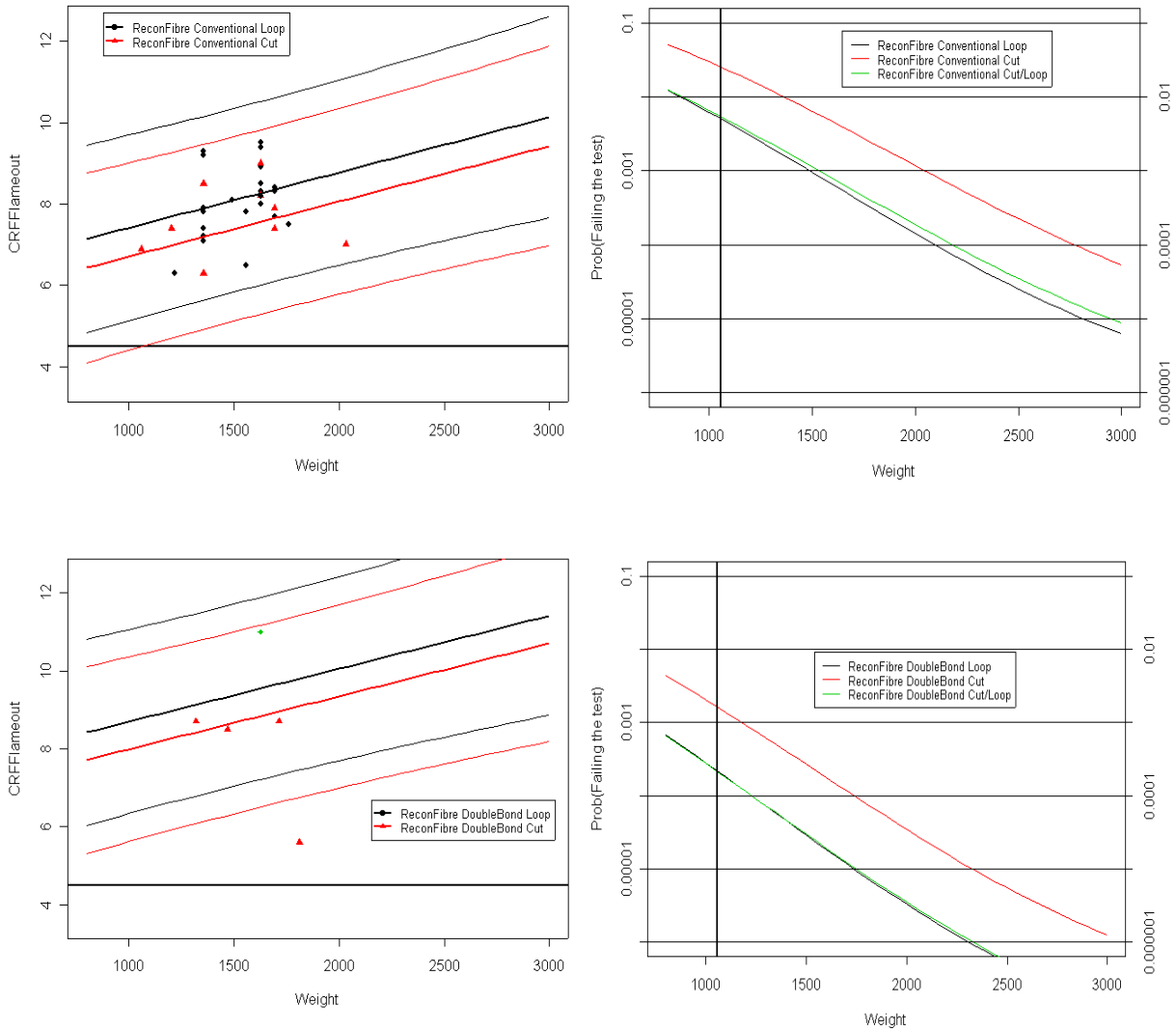
Figure 7-5: CRF vs Weight for Reconstituted Fibre with 95% prediction intervals, and probability of failing the CRF test at 4.5kW/m 2
